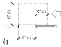
Side Approach-Hinge
